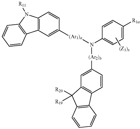
Formula 2A
