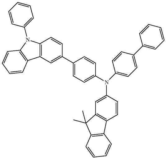
Compound 301
