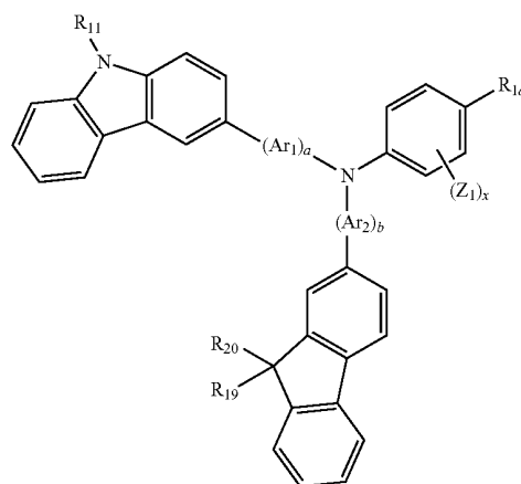
Formula 2B
