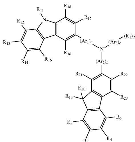
Formula 2
