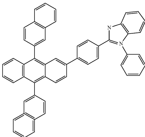
Compound 602
