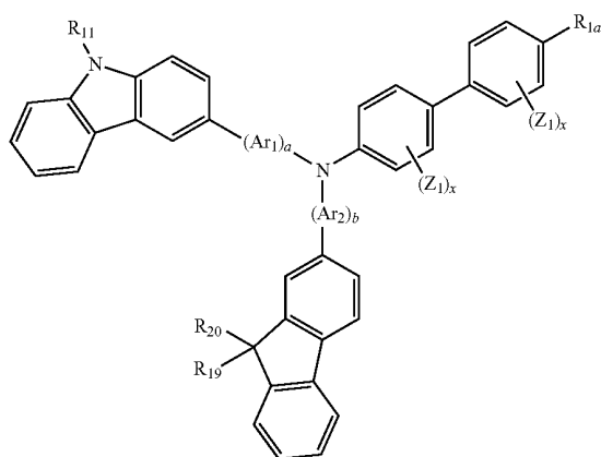
Formula 2K
