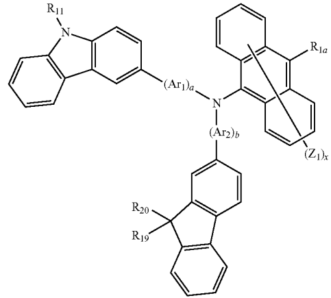
Formula 2J
